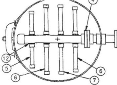
POSITION UNDERDRAIN LATERALS WITH SLOTS(.017") FACING BOTTOM OF TANK UNDERDRAIN SECTION
