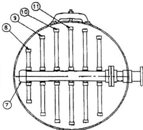
POSITION LATERALS (50 SLOTS) WITH SLOTS FACING TOP OF TANK OVERDRAIN SECTION
