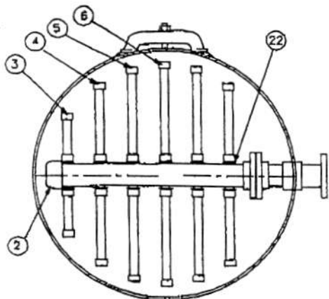
POSITION LATERALS (50 SLOTS) WITH SLOTS FACING BOTTOM OF TANK UNDERDRAIN SECTION
