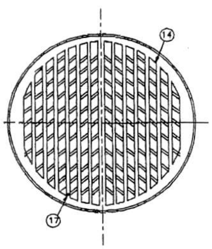
UPPER BAFFLE SYSTEM
