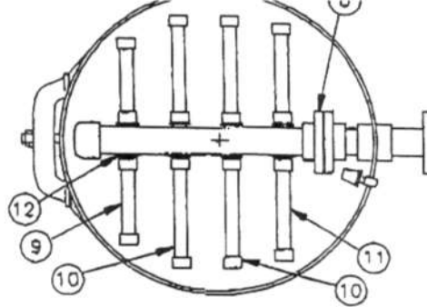
POSITION OVERDRAIN LATERALS WITH SLOTS(.50") FACING TOP OF TANK OVERDRAIN SECTION
